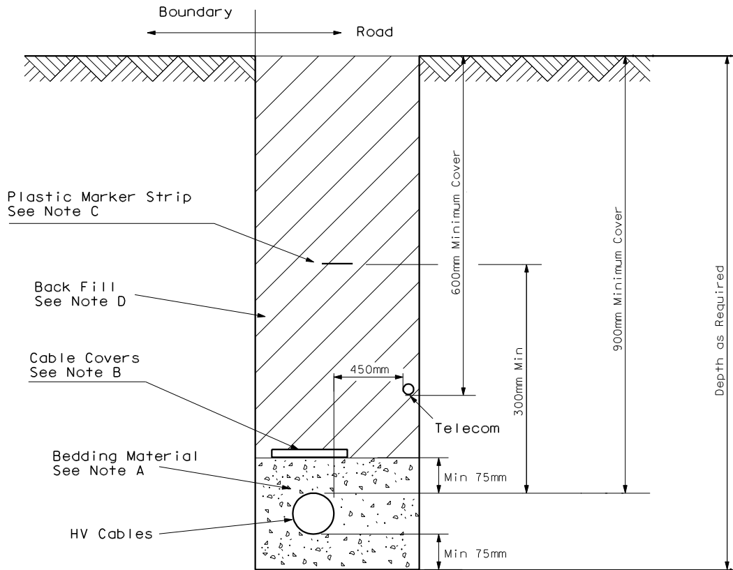
Directly Laid HV (with Telecom)
