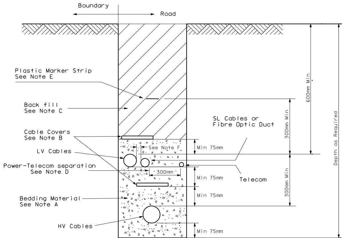
Directly Laid HV & LV Cable with Telecom
