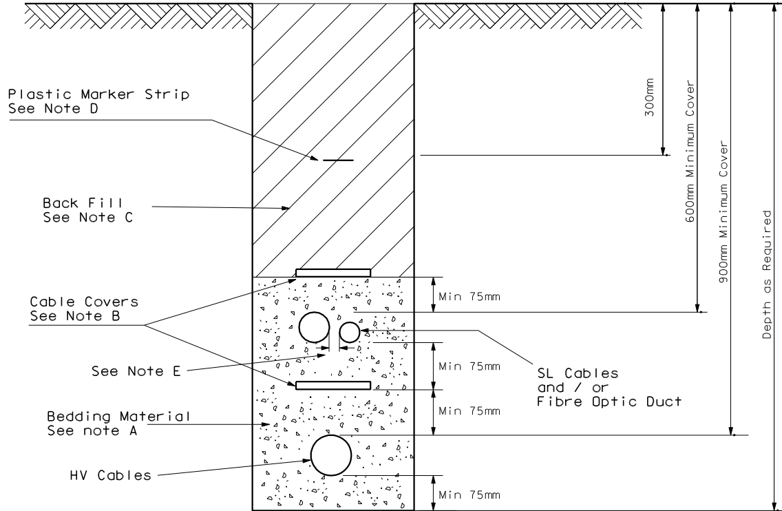
Directly Laid HV & LV Cables (or Spare Duct)
